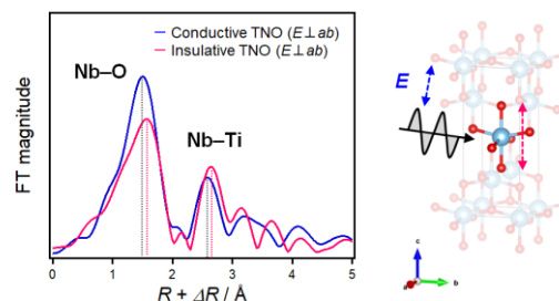
Fig. 1 Fourier-transformed (FT) magnitudes of k^3 -weighted Nb K -edge extended X-ray absorption fine structure signals for the (blue) as-deposited conductive and (red) after insulative Nb-doped TiO 2 thin films.
