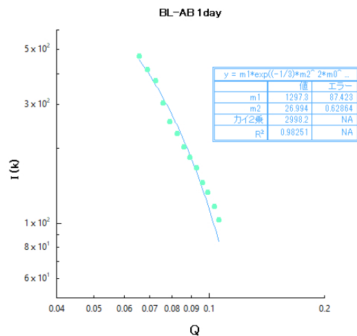
Fig.1 Typical Guinier fitting for bilayer film made by Type A and B gelatin.
